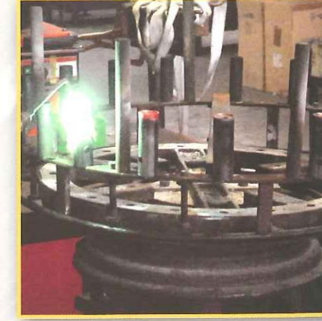
Saldatura gas flux Gas flux welding
