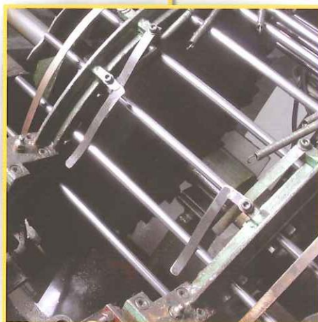
Filettatrice automatica Automatic threading-machine
