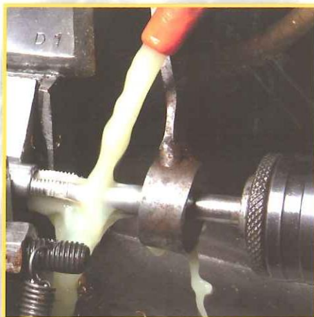
Maschiatrice Tapping-machine
