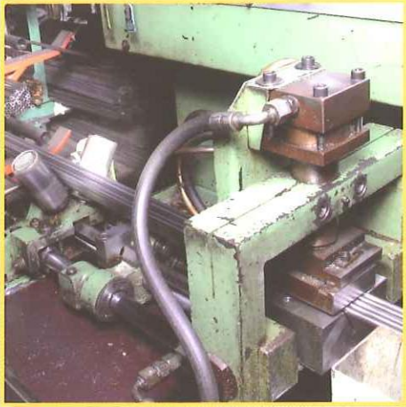
Troncatrice tubi Pipes cutting-machine
